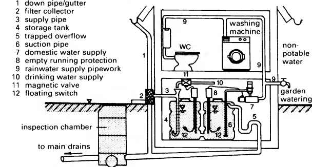
9 Rainwater system
